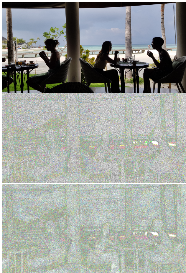
Figure A3. Example from CLIC.mobile, showing x , r and a sample from p(r) . White means zero residual.
