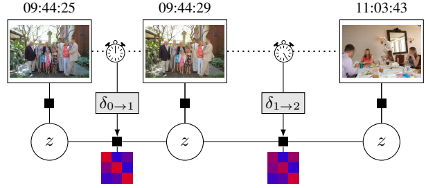
Figure 4: Illustration of our Stopwatch Hidden Markov model. The transition matrix between two consecutive images depends on the temporal gap \delta_{t \rightarrow t+1} . This allows to model bursts of photos and the typical durations of sub-events.
