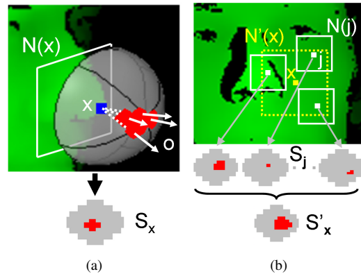
Figure 4. a) The single signature S_x is the set of orientations \mathbf{o} for which the pixel’s position \mathbf{x} is a maximum along \mathbf{o} compared to pixels in the neighborhood N(\mathbf{x}) . b) Single signatures S_j of points j in N'(\mathbf{x}) are merged into the aggregated signature S'_x .
