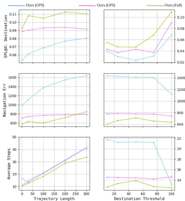
Fig. 9 Rows for metrics and columns for evaluation settings. Trajectory length: % extra length of path allowed for agents to navigate at evaluation. Destination Threshold (meter): a threshold of the final distance to the destination, below which is considered as a success
